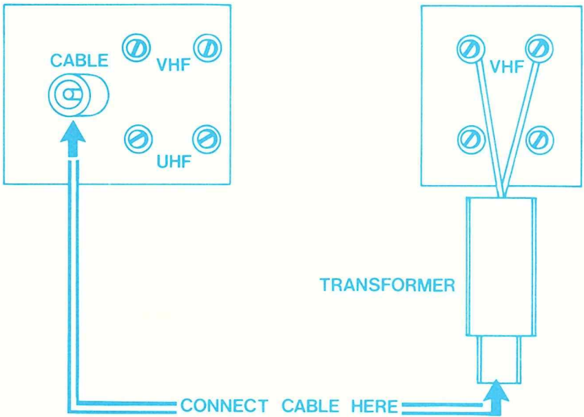
Typical TV Connections
